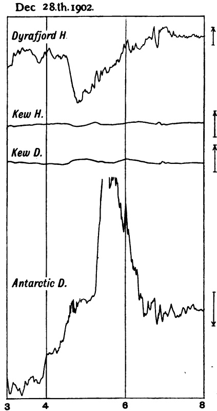
FIG. 37.—ARCTIC-KEW-ANTARCTIC CURVES.
